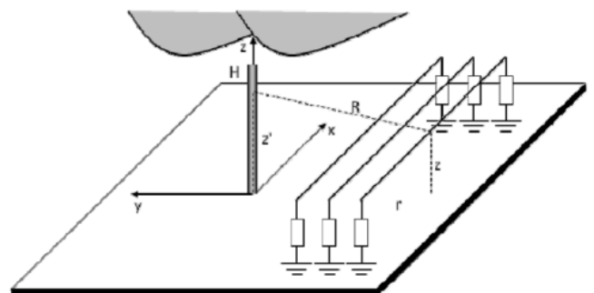
Fig.1. Geometry used to calculate the induced lightning overvoltage on a multiconductor overhead line
